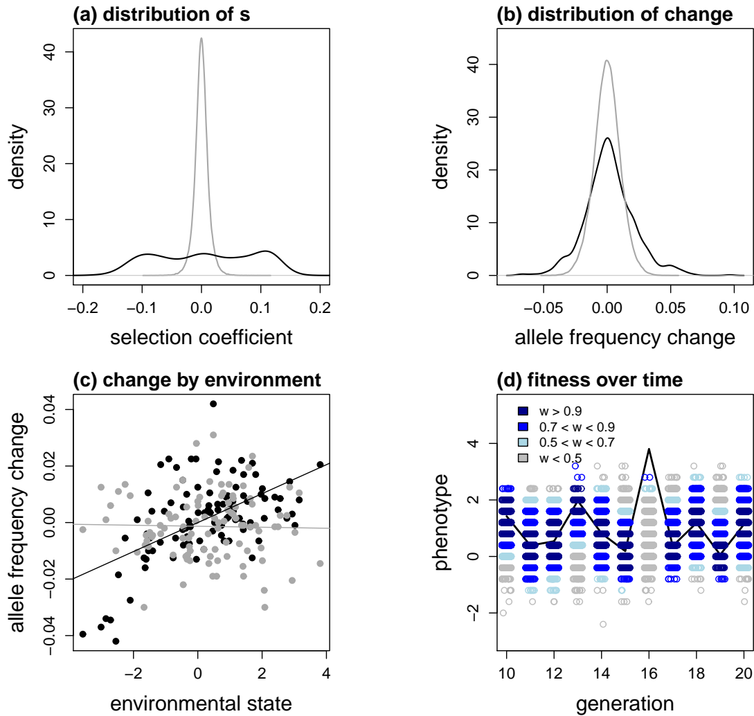
Figure 4: These plots summarize patterns of selection and allele frequency change for one of the five quantiNEMO simulations. (a) Density plots depict the distribution of the actual selection experienced by neutral (gray) and non-neutral (black) loci. These selection coefficients capture the effects of direct and indirect selection. (b) Density plots depict the distribution of allele frequency change between generations at neutral (gray) and non-neutral (black) loci. (c) A scatterplot shows the relationship between the environmental state and allele frequency change at neutral (gray) and non-neutral (black) loci. The solid lines show the inferred relationship from linear regression. (d) Points indicate the expected fitness of each individual each generation in a single population. Points were jittered along the x-axis to improve visualization. A line shows the optimal phenotypic value each generation based on the state of the environment.
