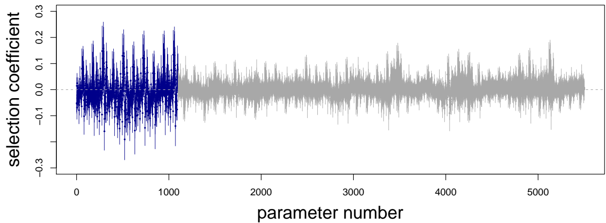
Figure 5: The plot summarize the posterior probability distributions for selection coefficients for one of the data sets generated with quantinemo . Gray (neutral loci) or blue (non-neutral loci) points and lines indicate the posterior median and 95% ETPIs for the selection coefficients for specific loci, populations, and generations. All 110 population by generation combinations are shown for the ten non-neutral loci, and for a subset of forty representative neutral loci.
