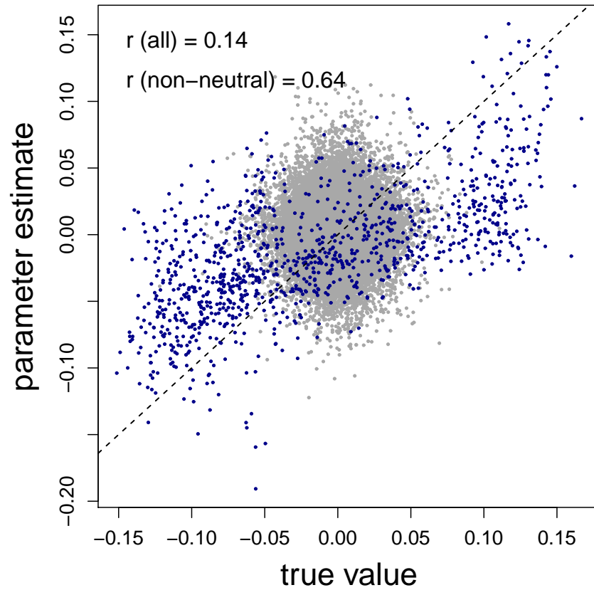
Figure 6: This scatterplot shows the relationship between the true and estimated selection experienced by each locus for one of the five fluctuating selection data sets simulated with quantinEMO . This includes direct selection and indirect selection caused by statistical associations between neutral and non-neutral loci. Neutral loci are shown in gray and non-neutral loci are shown in blue. A dashed black line shows the expected one-to-one relationship. Correlation coefficients between true and estimated values for this data set are reported for all loci and for the subset of non-neutral loci.
