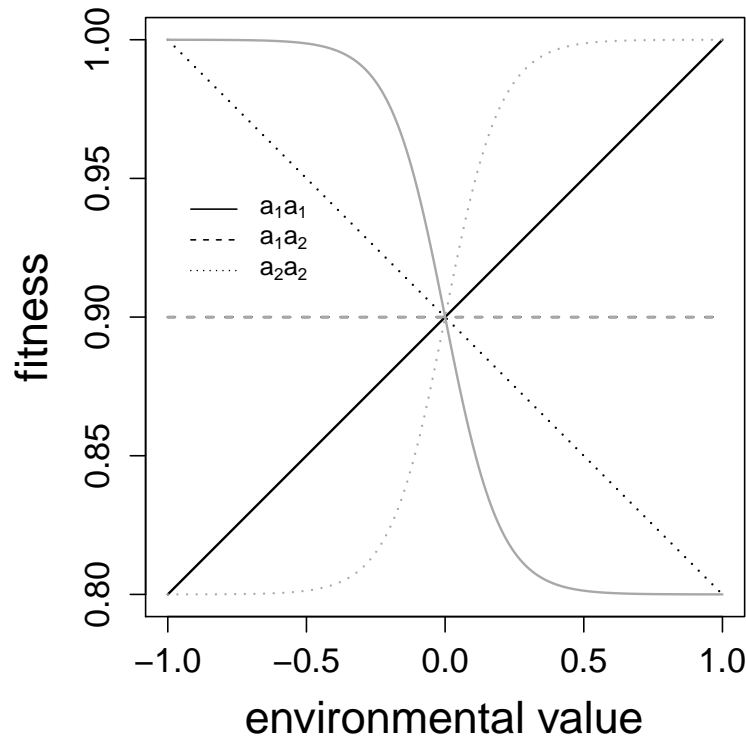
Figure 2: Lines in this plot show the fitness functions used for the Wright Fisher simulations with linear (black) and non-linear (gray) fluctuating selection. A logistic function with a slope of \pm 10 was used to model non-linear selection. No genotype had a net fitness advantage, but rather alternative homozygotes performed better in different environments. Heterozygotes had a constant and intermediate fitness in all Wright Fisher simulations and across all environments.
