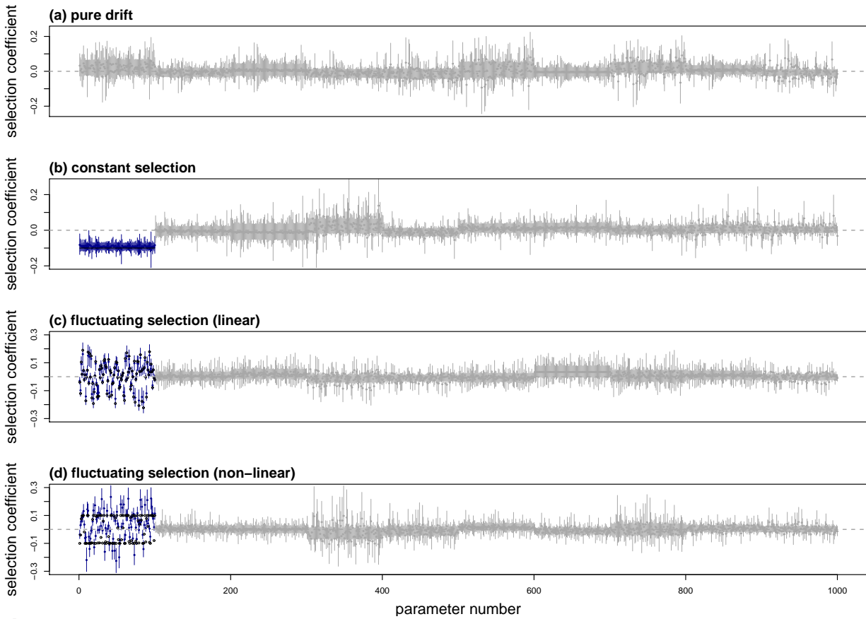
Figure 3: These plots summarize the posterior probability distributions of selection coefficients for different simulated data sets. Gray (neutral loci) or blue (non-neutral loci) points and lines indicate the posterior median and 95% ETPIs for the selection coefficients for specific loci, populations, and generations. All 100 population by generation combinations are shown for the non-neutral locus, and for a subset of nine representative neutral loci. The true value of s is indicated by a black line (constant selection) or black points (fluctuating selection).
